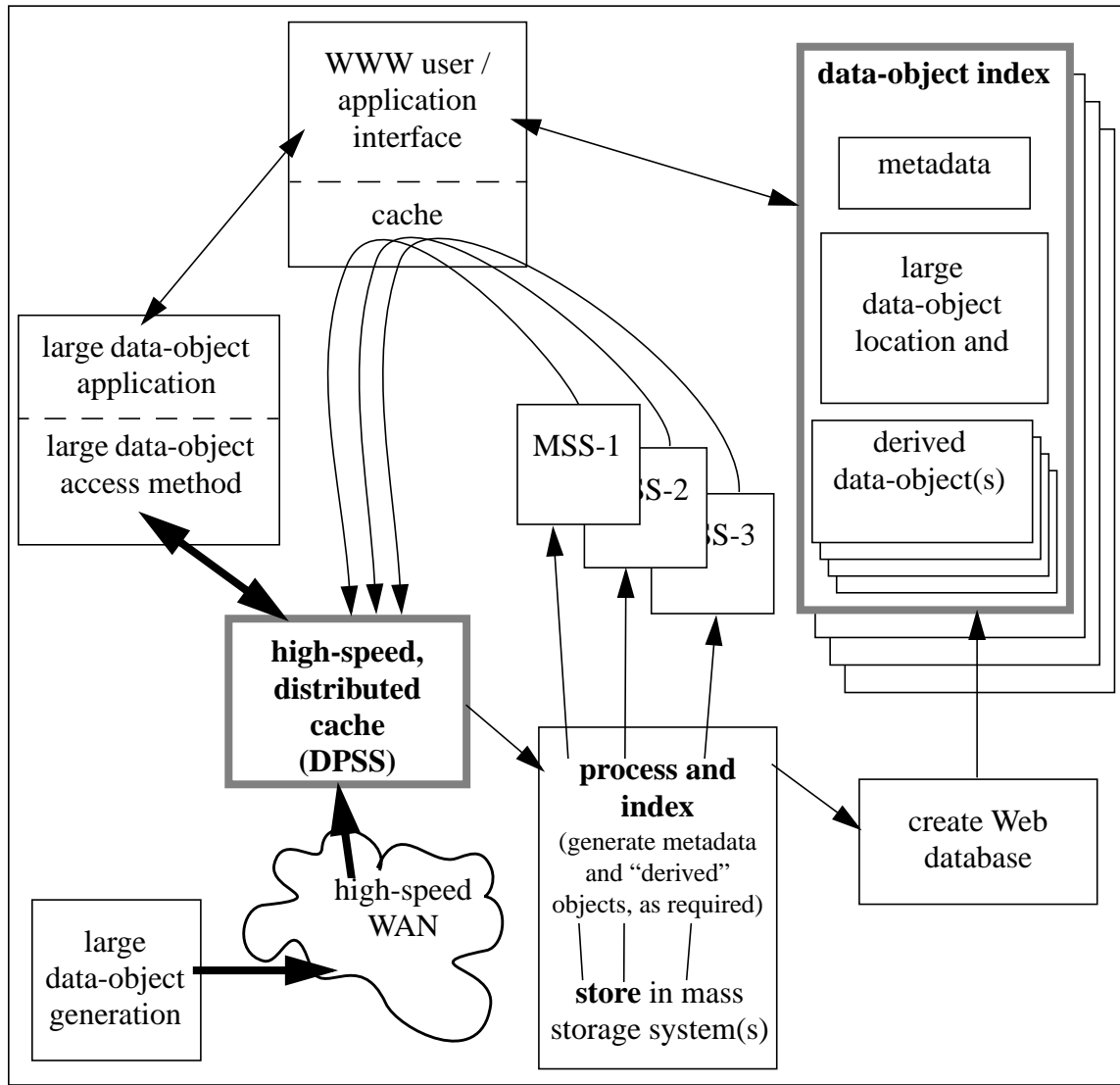
Figure 1 Overall Architecture for a Distributed, Large Data-Object Environment
