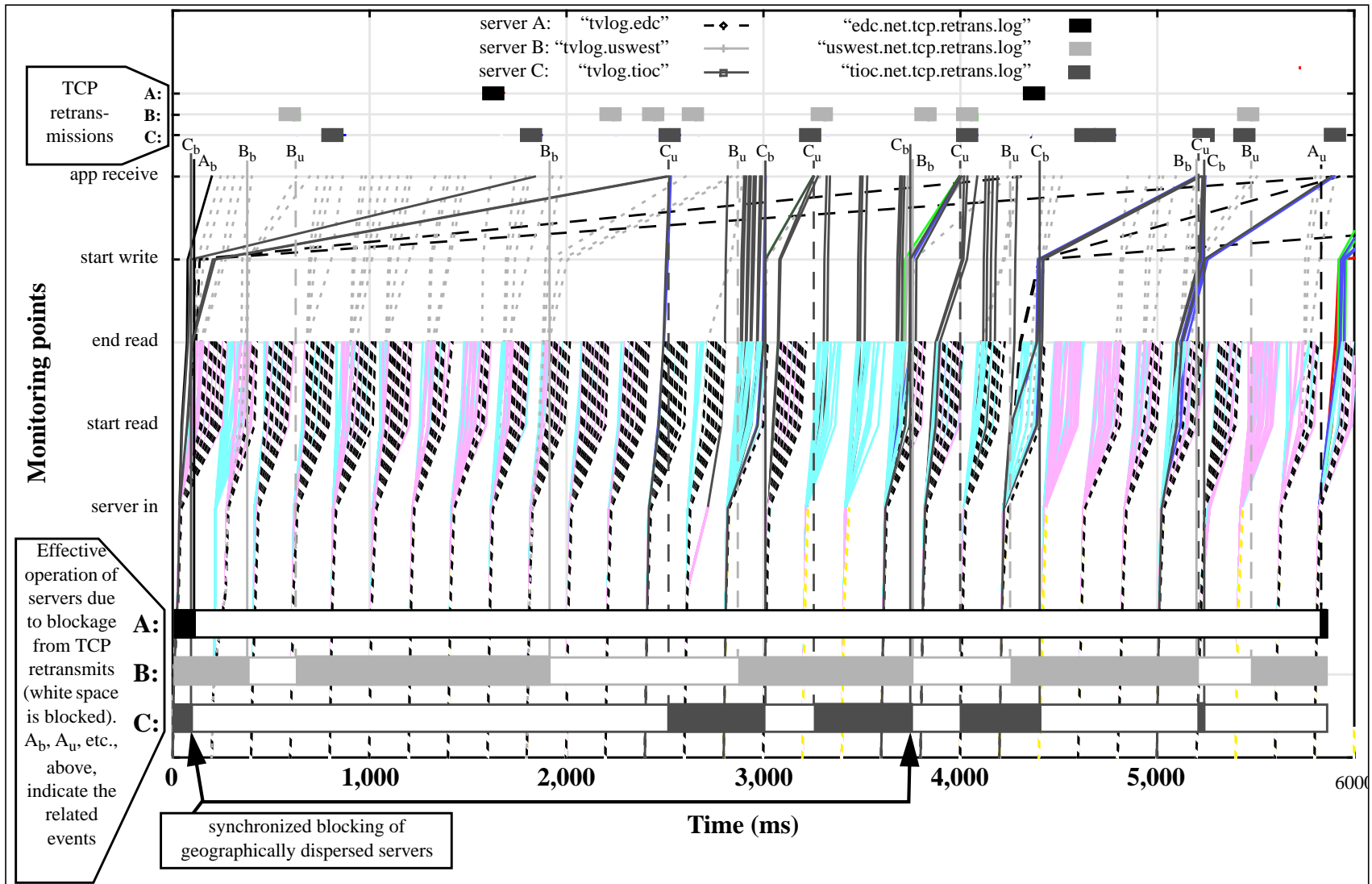
Figure 10 Three Server Test (MAGIC ATM WAN, three SS-10s as servers, tv_sim on SGI Onyx)
