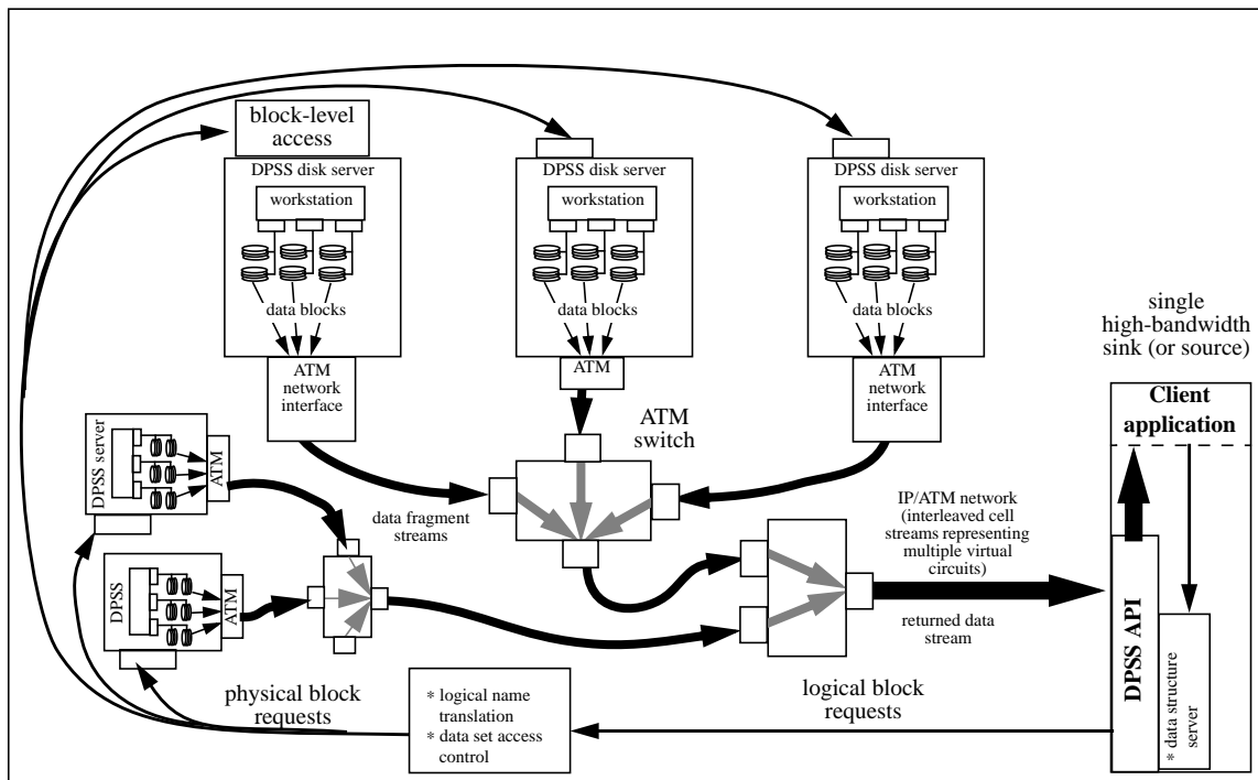
Figure 2 Distributed-Parallel Storage System Implementation
