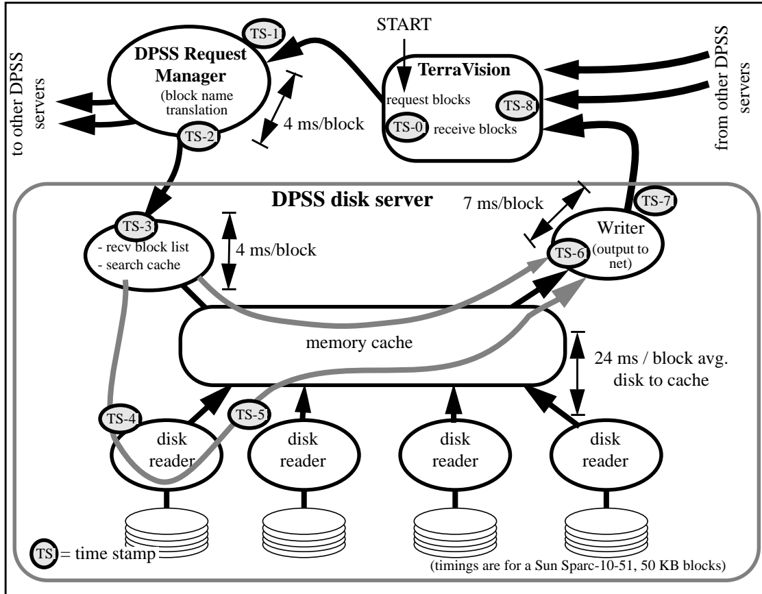
Figure 5 DPSS Performance Characterization Points and Optimal Average Timings
