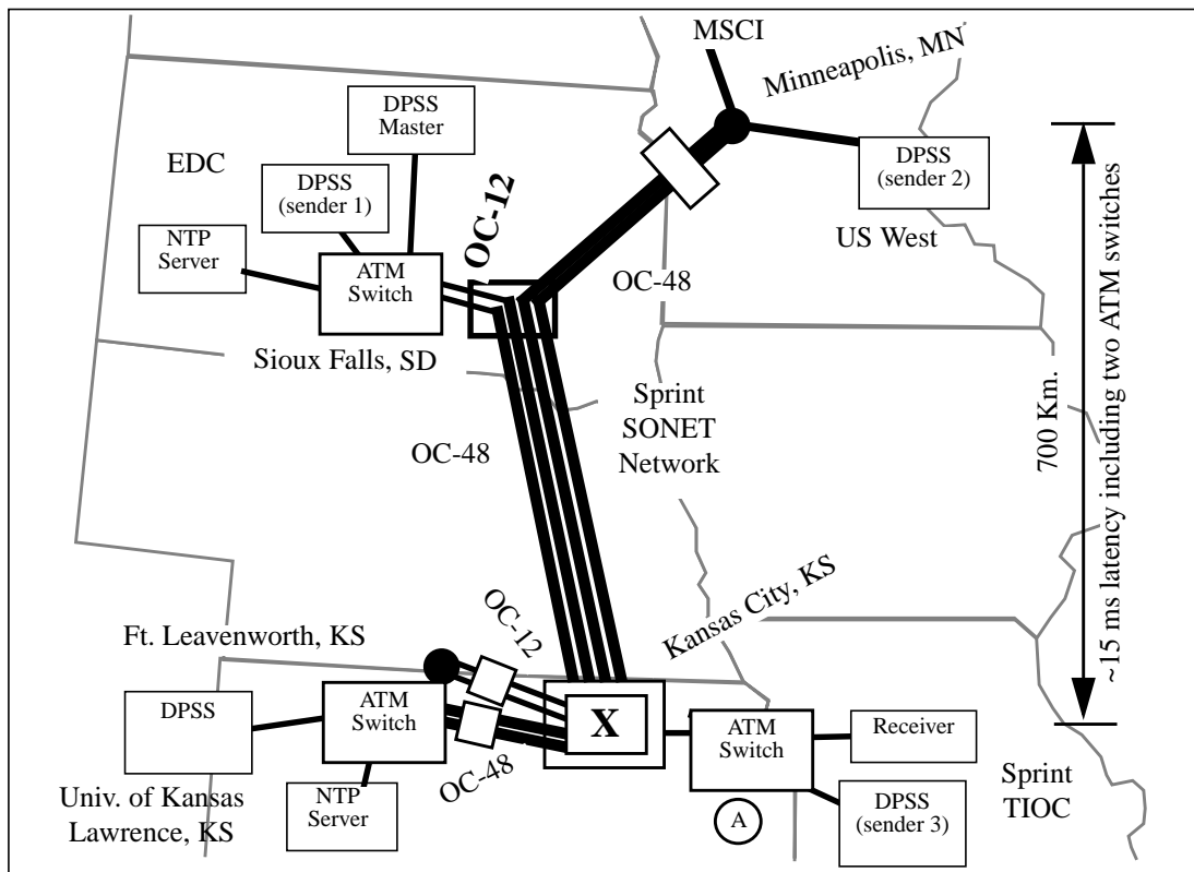
Figure 9 The MAGIC Network: Test Configuration
